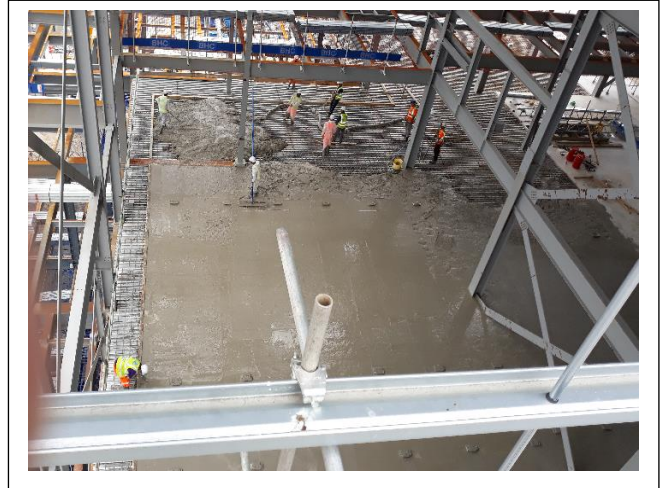
Phase 3A first floor concrete pour.
